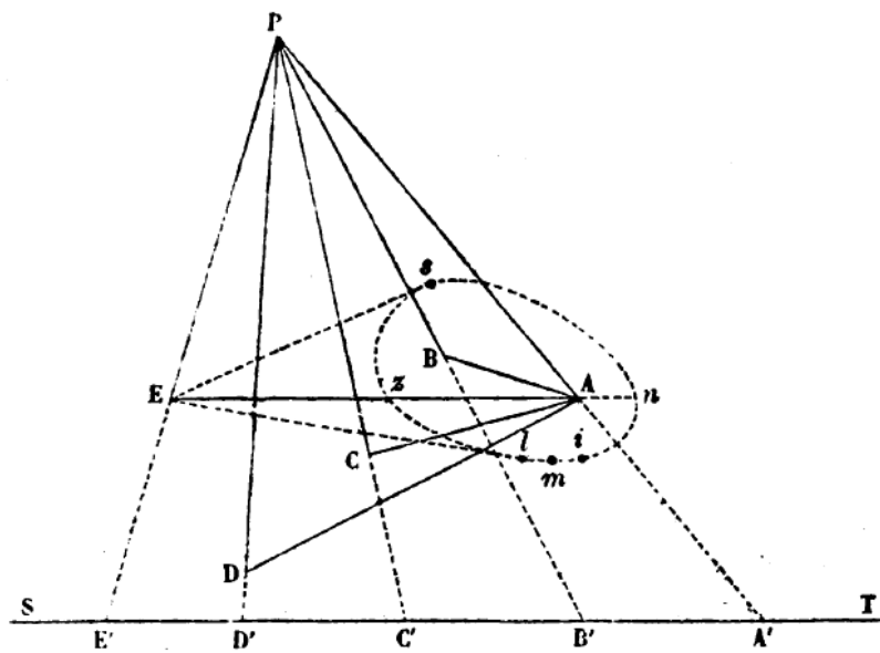
Figure 5.12: Mourey's geometrical interpretation of the F.T.A. 379
