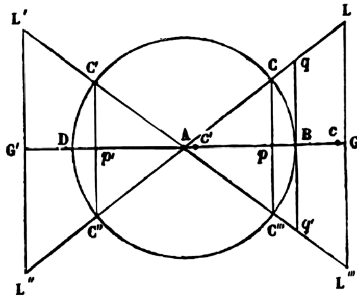
Figure 5.11: Relating trigonometric lines and paths. 368
