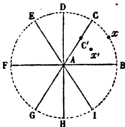
Figure 5.9: The directed angle. 351
